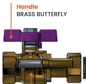
Body, ball, connections, shaft and metal parts Brass CW617N, EN 12165 and 12164
